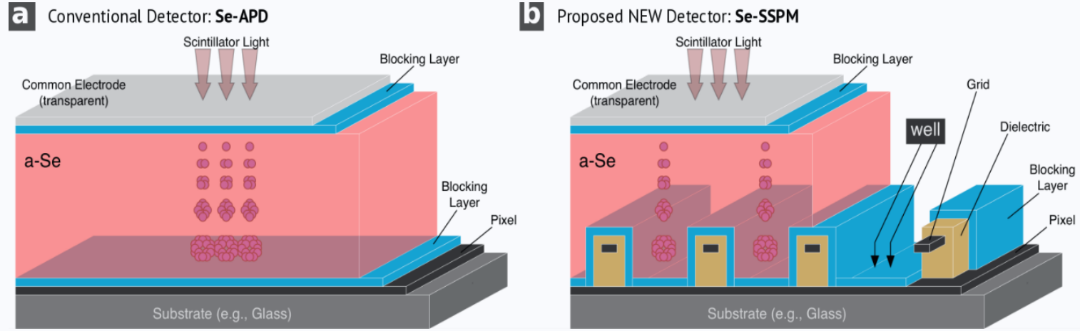
(a) Conventional planar a-Se detector. (b) Proposed NEW-HARP detector.
