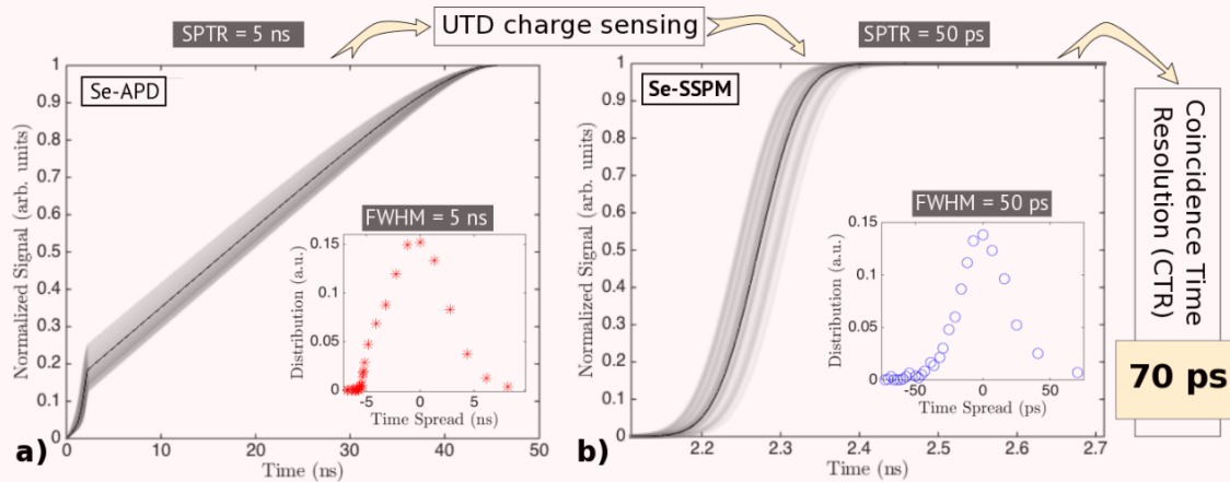
Simulation of signal gain over time for (a) conventional planar a-Se detector and (b) NEW-HARP.
