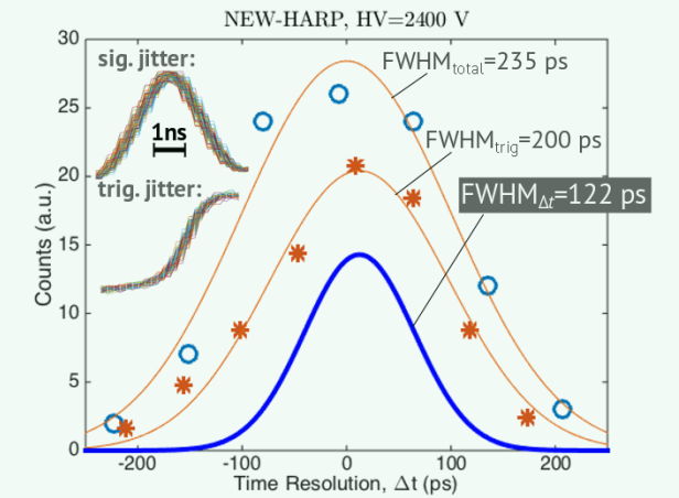
Experimental results for NEW-HARP SPTR.
