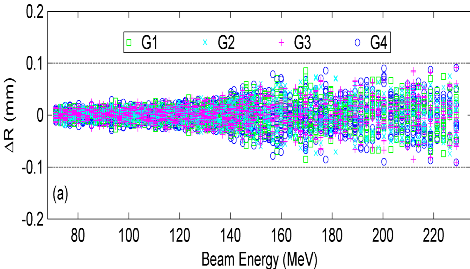
Fig 2. The range reproducibility ( \Delta R ) for all four gantry rooms (G1-G4)
