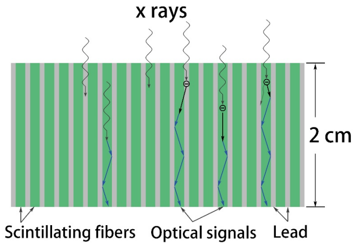
Detector design (cross section)
