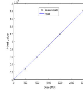
Dose Calibration
