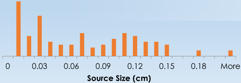
Pinnacle: Effective Source Size (X)
