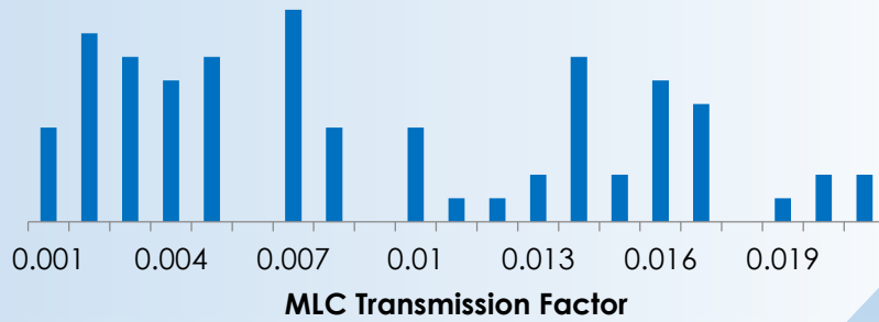
Pinnacle: MLC Transmission Factor
