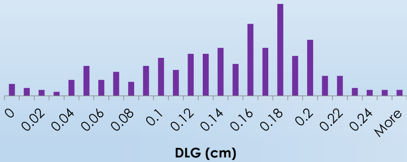
Eclipse: Dosimetric Leaf Gap
